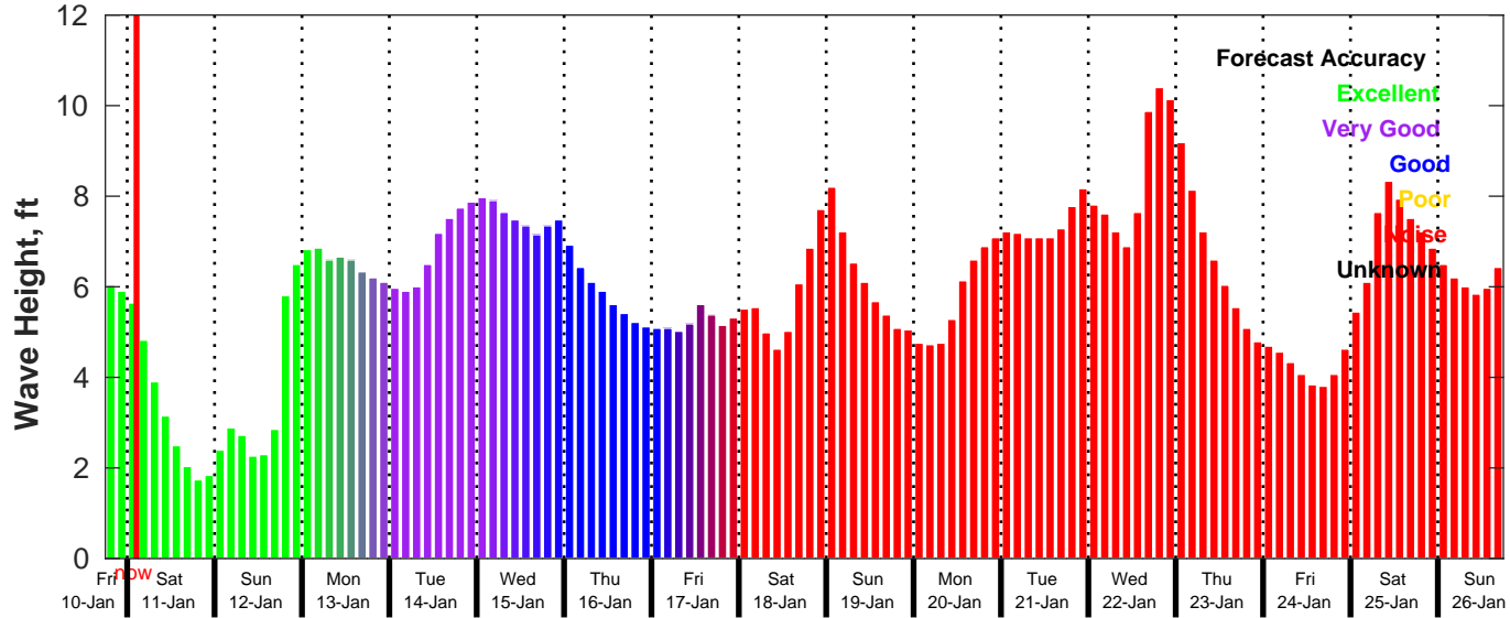
GFS Wave Forecast for NDBC 42020 from 10-Jan-2025 18:00:00 to 26-Jan-2025 18:00:00
