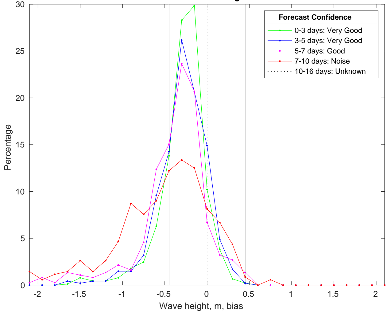
NDBC 42035 vs CMEMSWaves Bias Histogram: 11-Jan-2025
