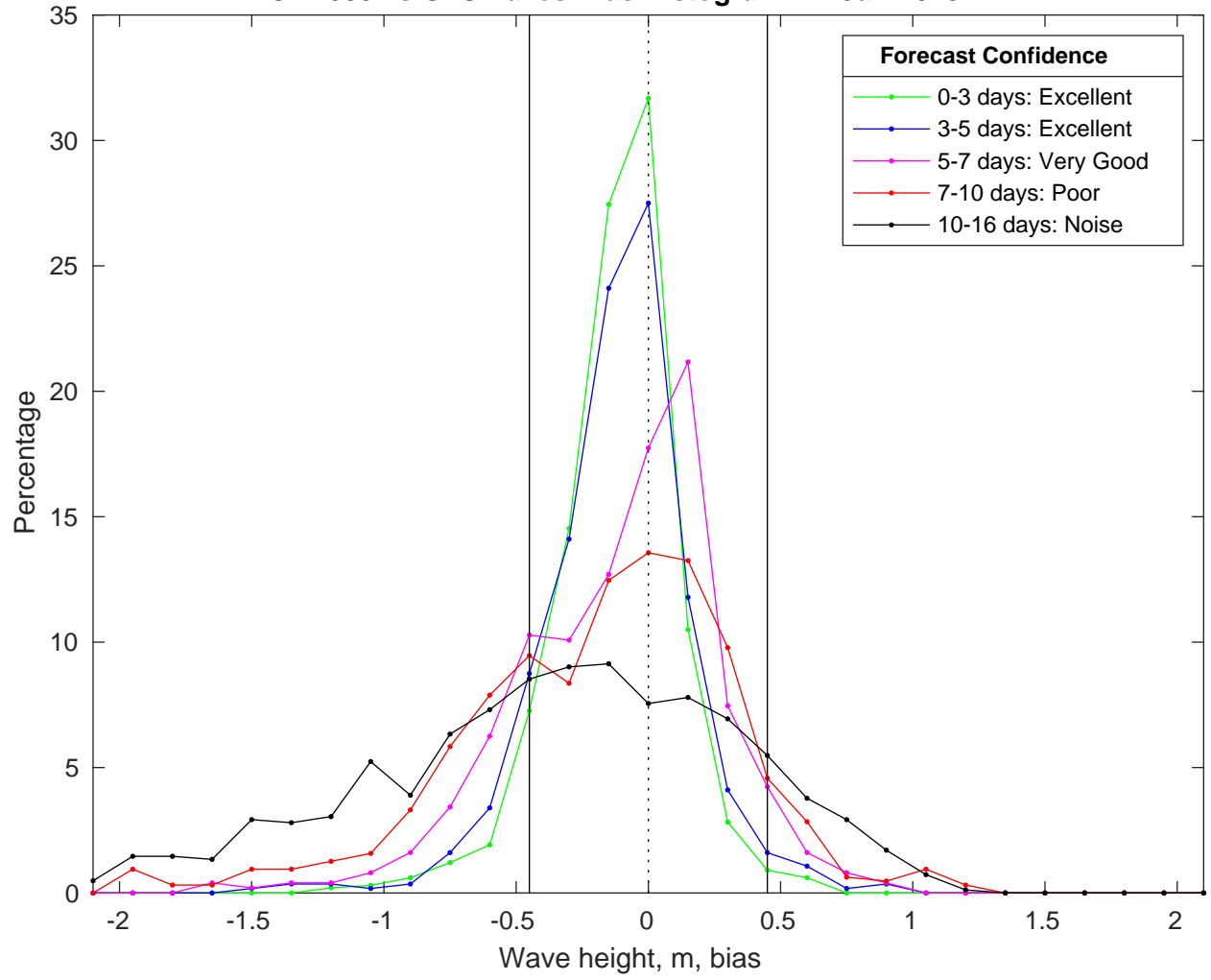
NDBC 42035 vs GFSWaves Bias Histogram: 11-Jan-2025
