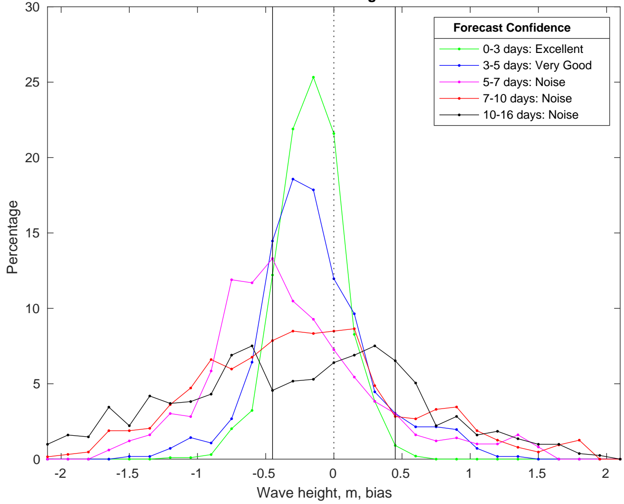
NDBC 42036 vs GFSWaves Bias Histogram: 11-Jan-2025
