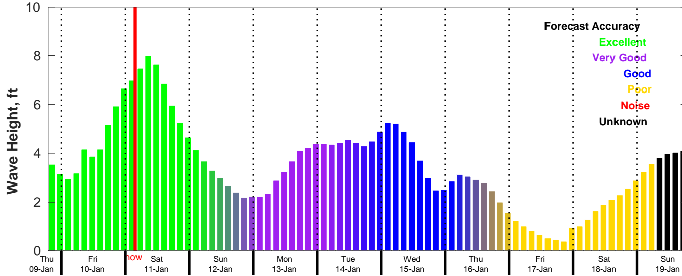
CMEMS Wave Forecast for NDBC 42036 from 09-Jan-2025 19:00:00 to 19-Jan-2025 19:00:00
