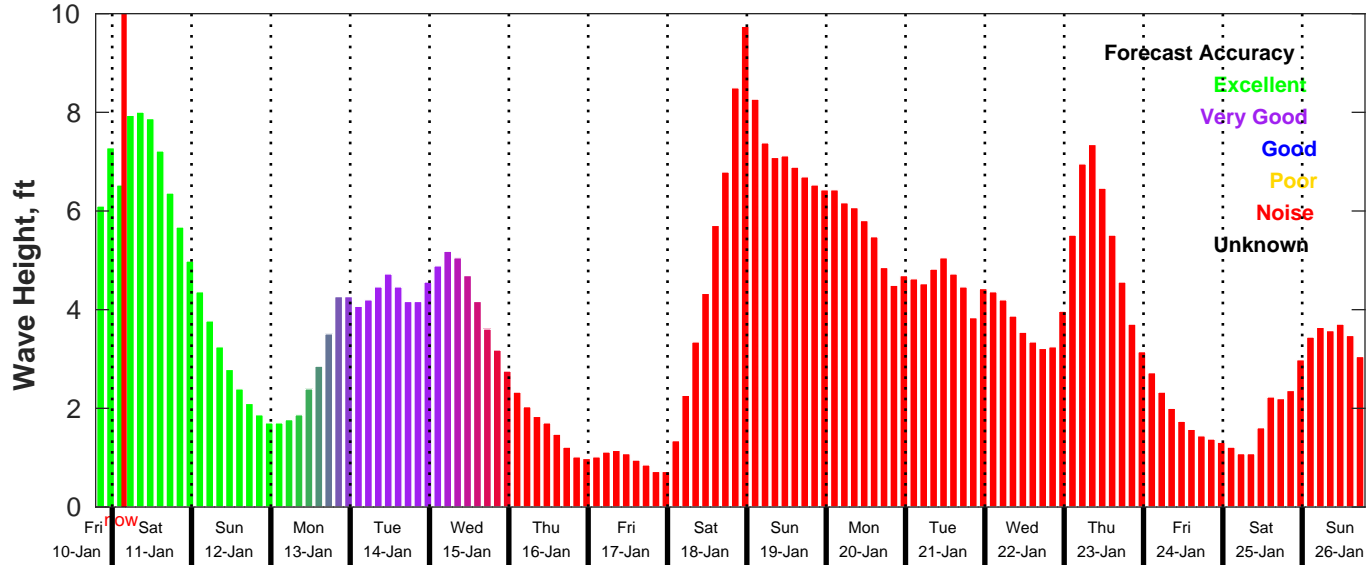
GFS Wave Forecast for NDBC 42036 from 10-Jan-2025 19:00:00 to 26-Jan-2025 19:00:00
