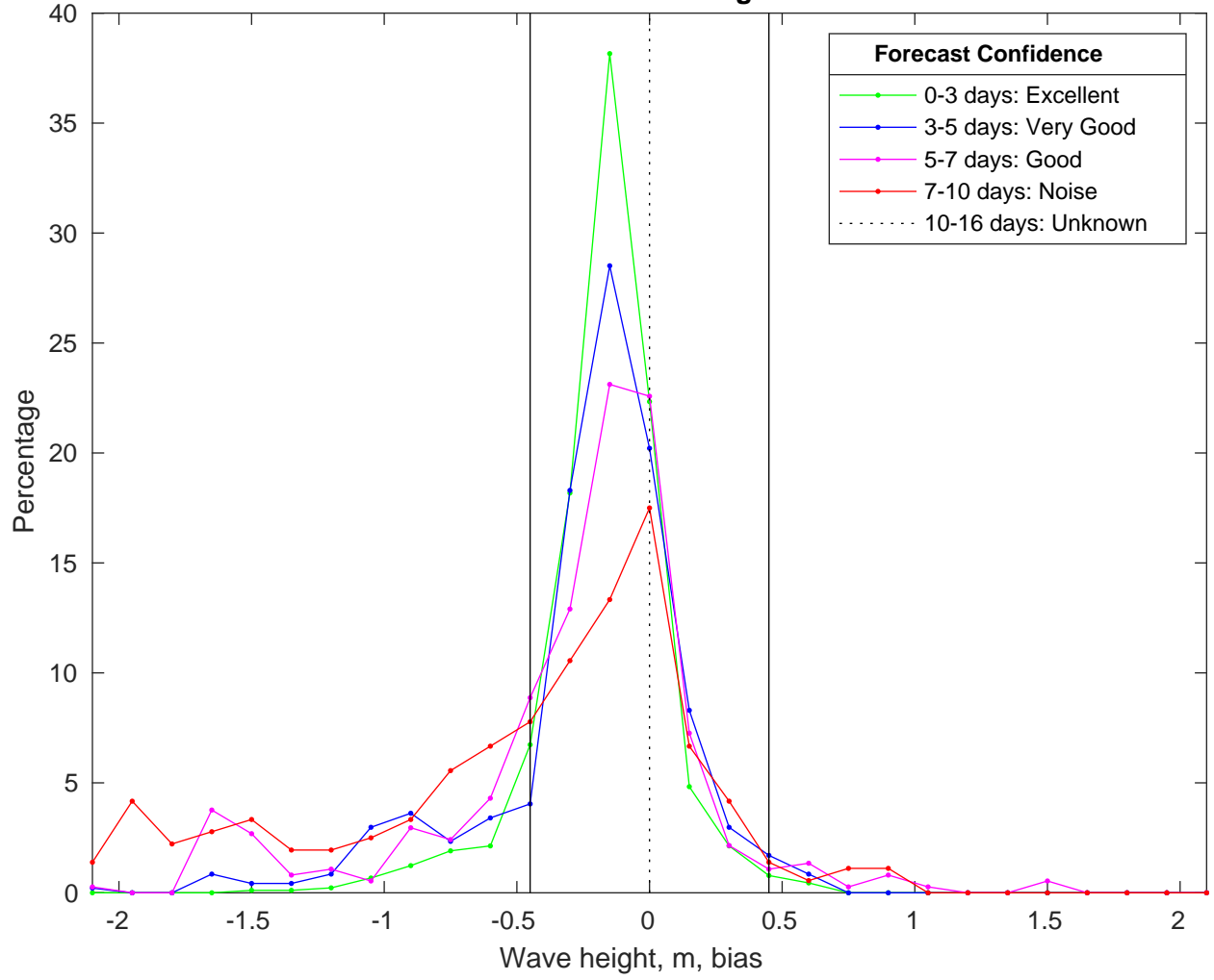
NDBC 42040 vs CMEMSWaves Bias Histogram: 11-Jan-2025
