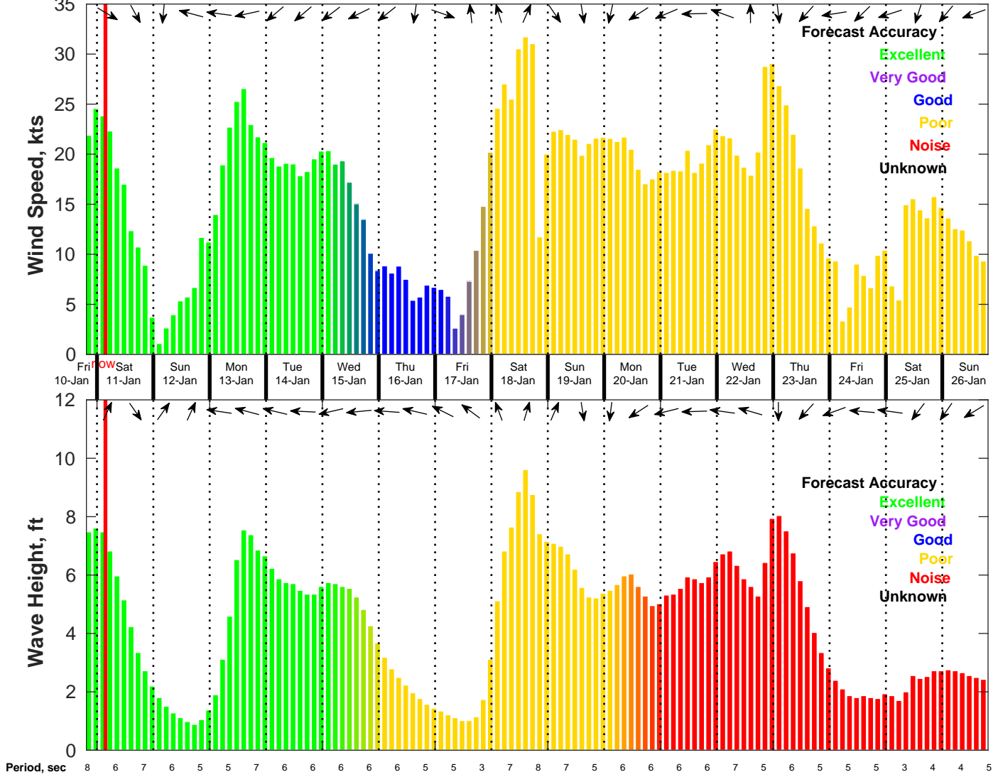
Wind & Wave Forecast for NDBC 42040 from 10-Jan-2025 19:00:00 to 26-Jan-2025 19:00:00
