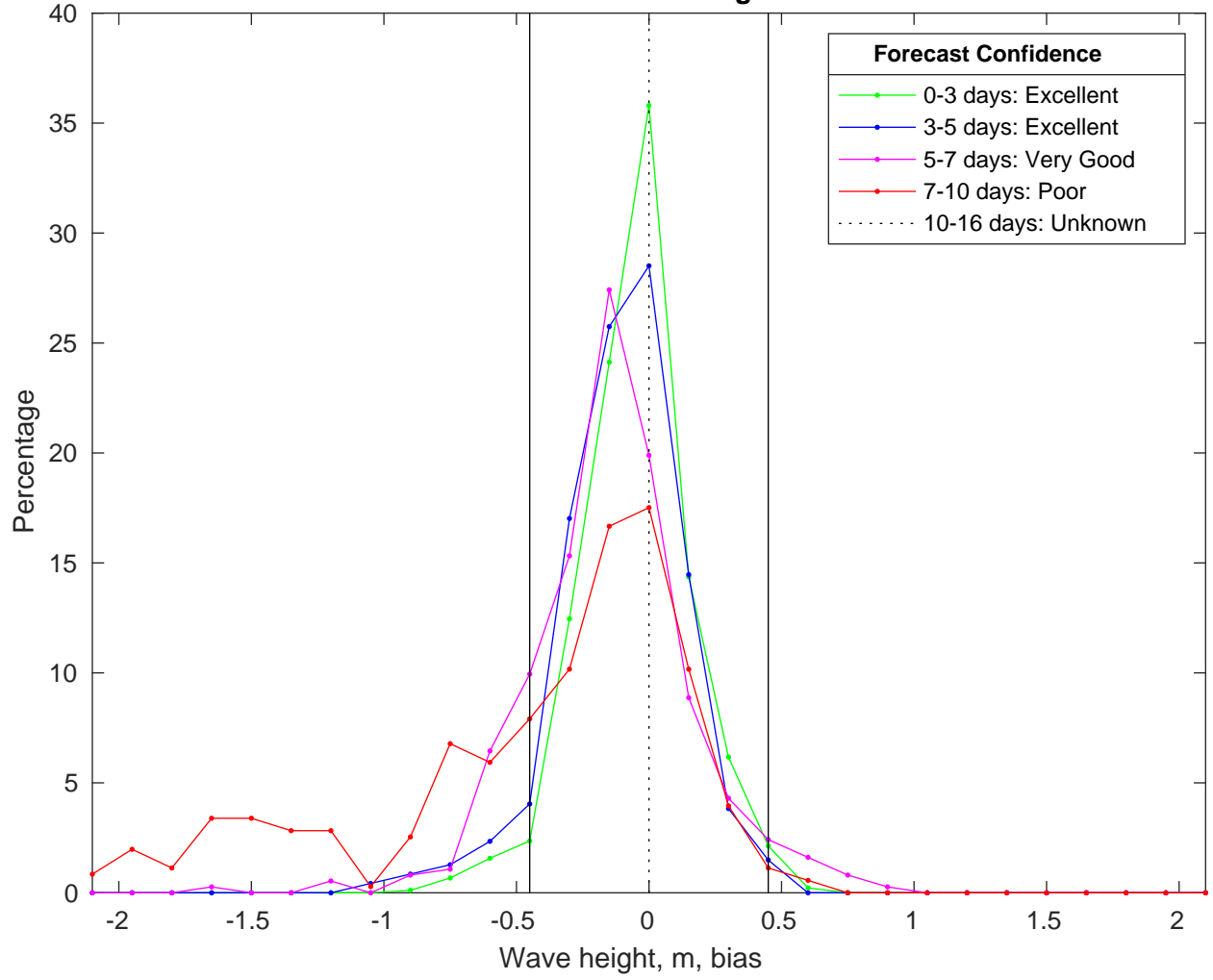
NDBC 42084 vs CMEMSWaves Bias Histogram: 11-Jan-2025
