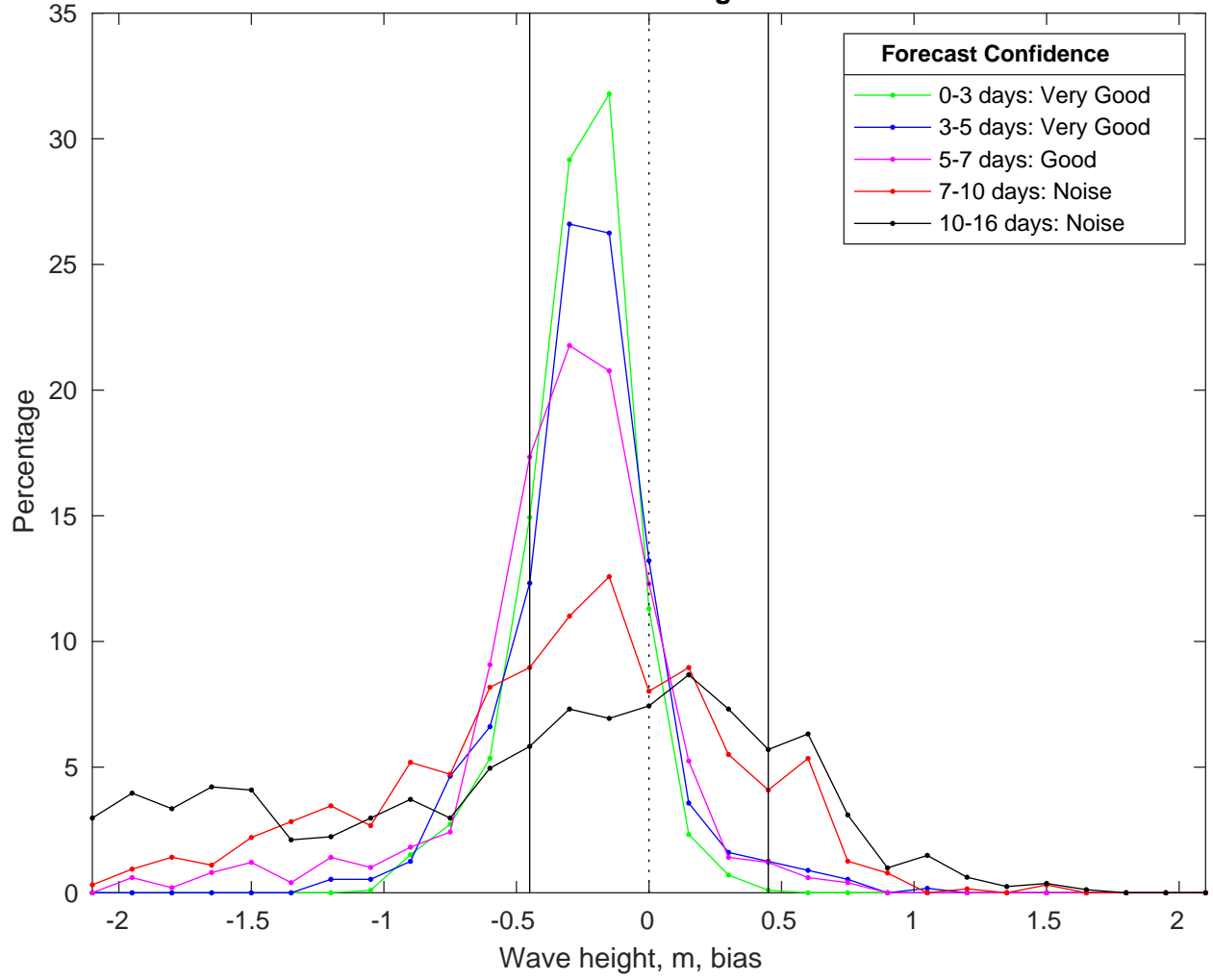
NDBC 42084 vs GFSWaves Bias Histogram: 11-Jan-2025
