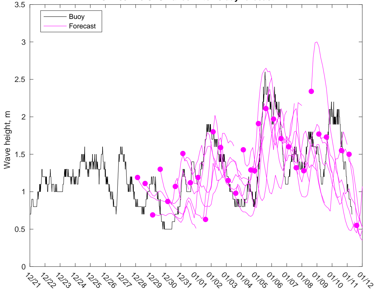
NDBC 42092 vs GFSWaves: 7 to 10 day forecast
