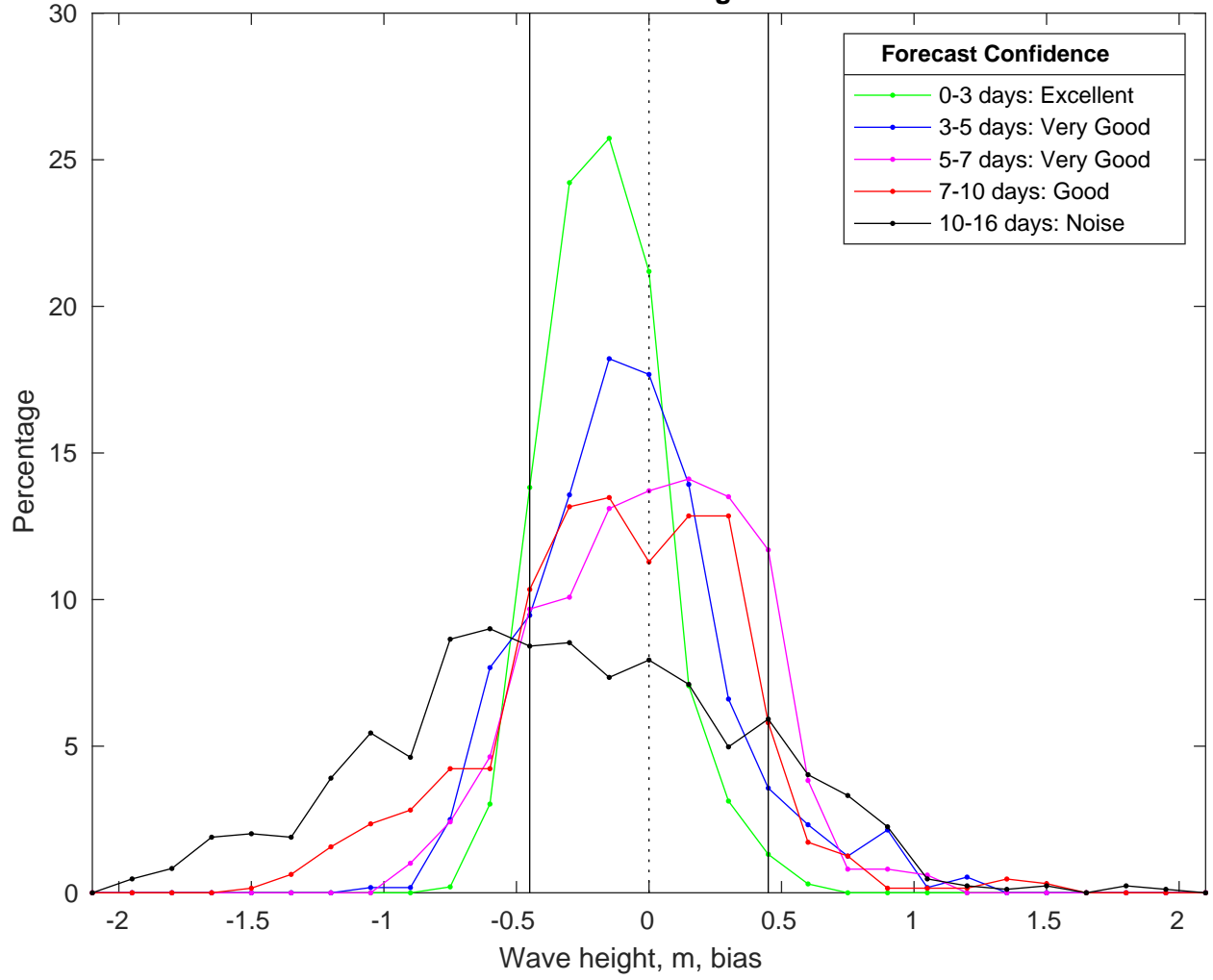
NDBC 42092 vs GFSWaves Bias Histogram: 11-Jan-2025
