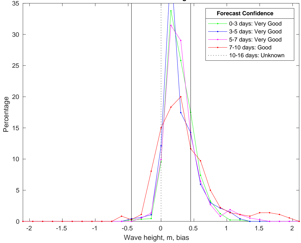
NDBC 44020 vs CMEMSWaves Bias Histogram: 11-Jan-2025
