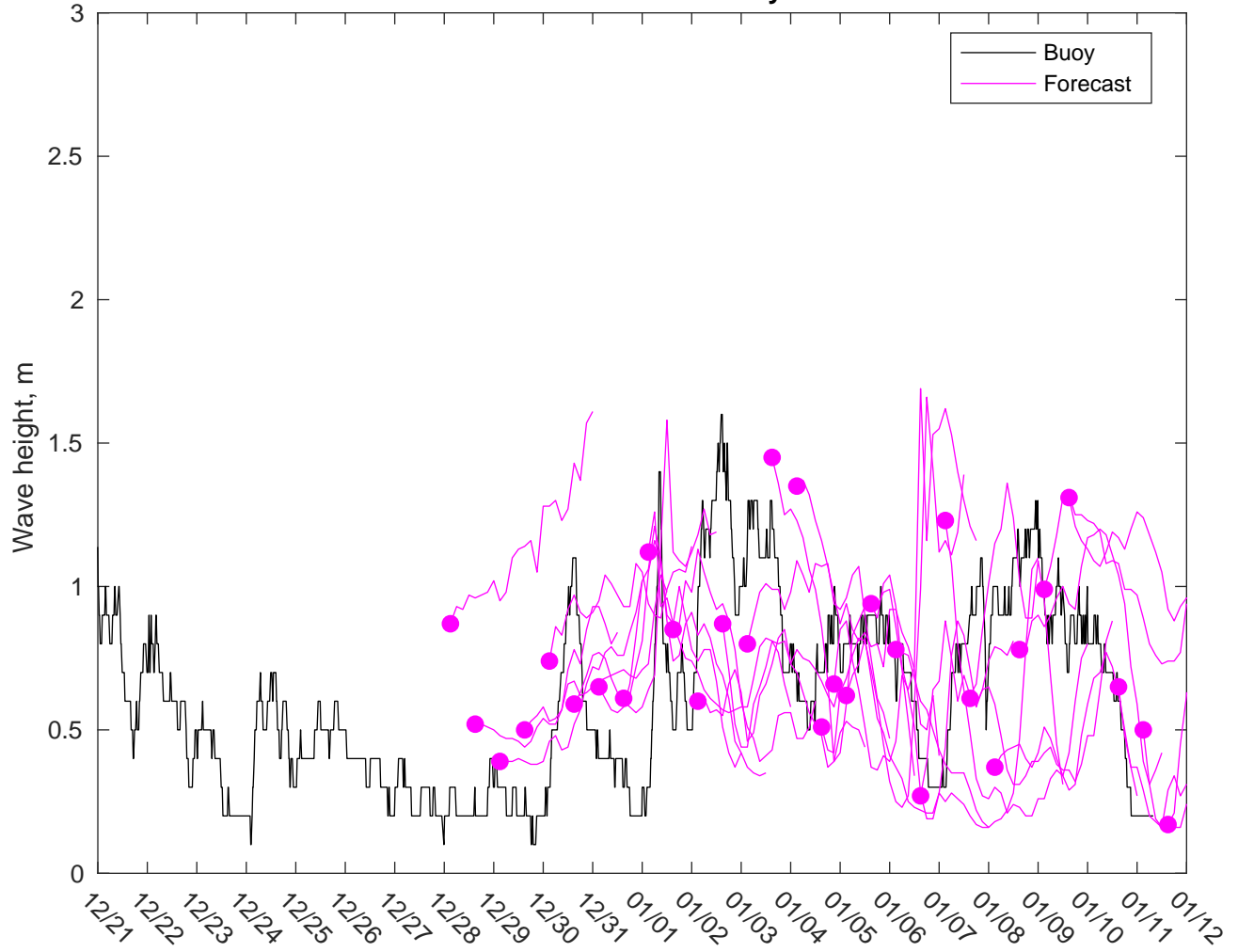
NDBC 44020 vs GFSWaves: 7 to 10 day forecast
