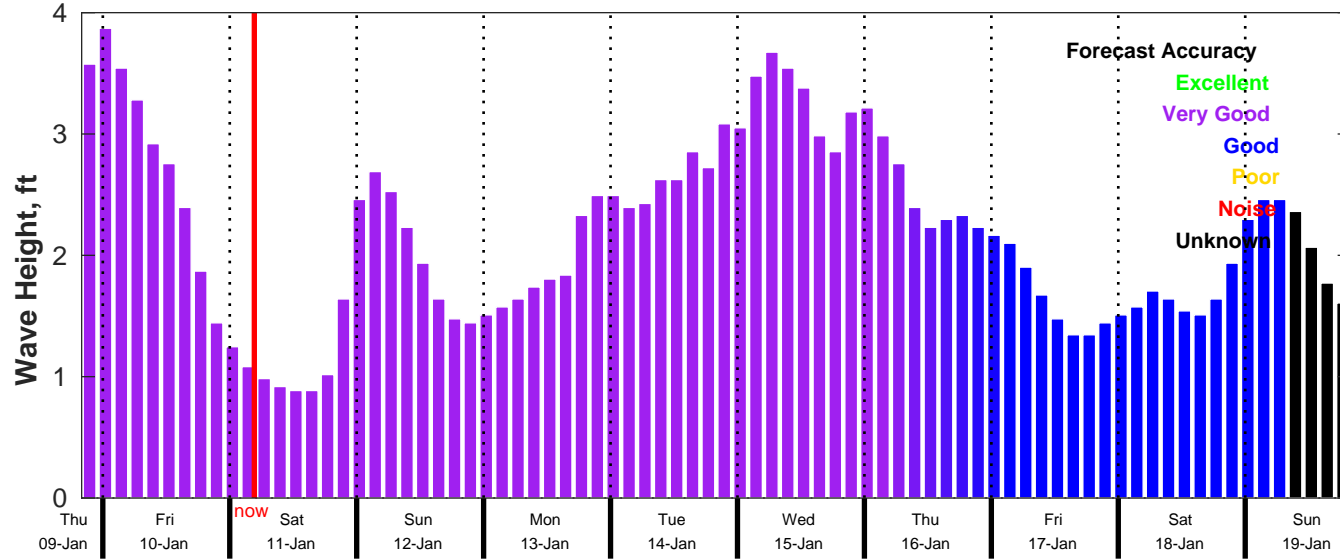
CMEMS Wave Forecast for NDBC 44020 from 09-Jan-2025 20:00:00 to 19-Jan-2025 20:00:00
