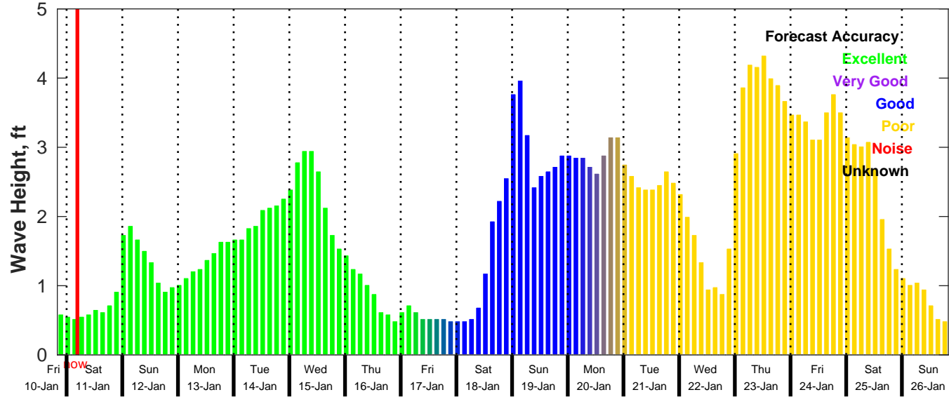
GFS Wave Forecast for NDBC 44020 from 10-Jan-2025 20:00:00 to 26-Jan-2025 20:00:00
