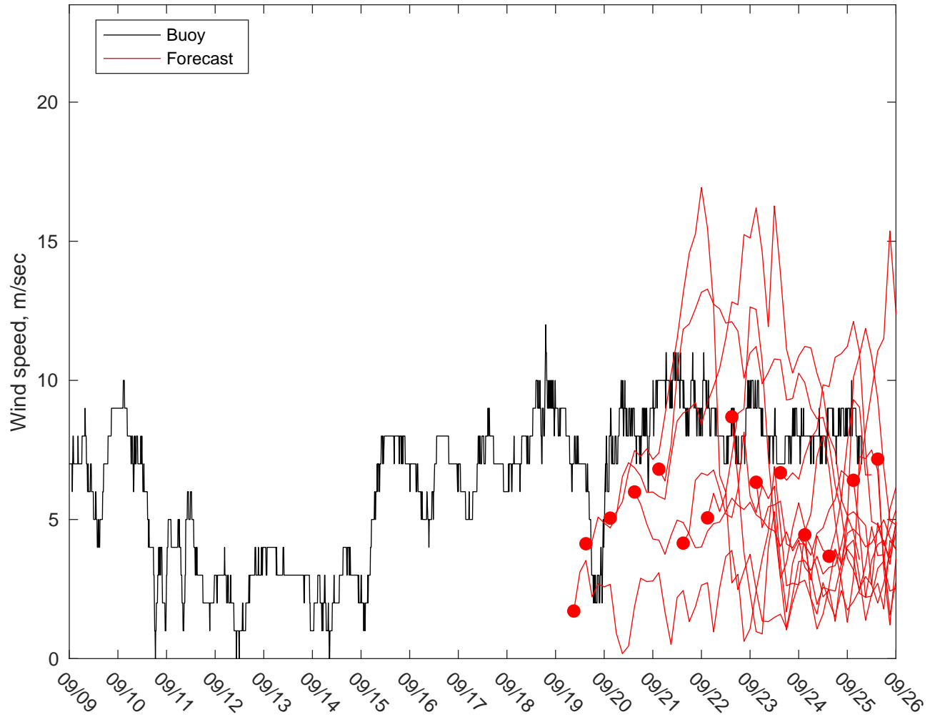
NDBC 44025 vs GFSWinds: 10 to 16 day forecast
