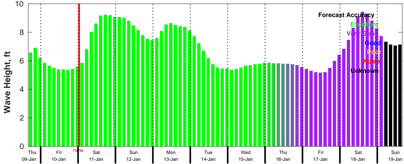
CMEMS Wave Forecast for NDBC 46011 from 09-Jan-2025 16:00:00 to 19-Jan-2025 16:00:00
