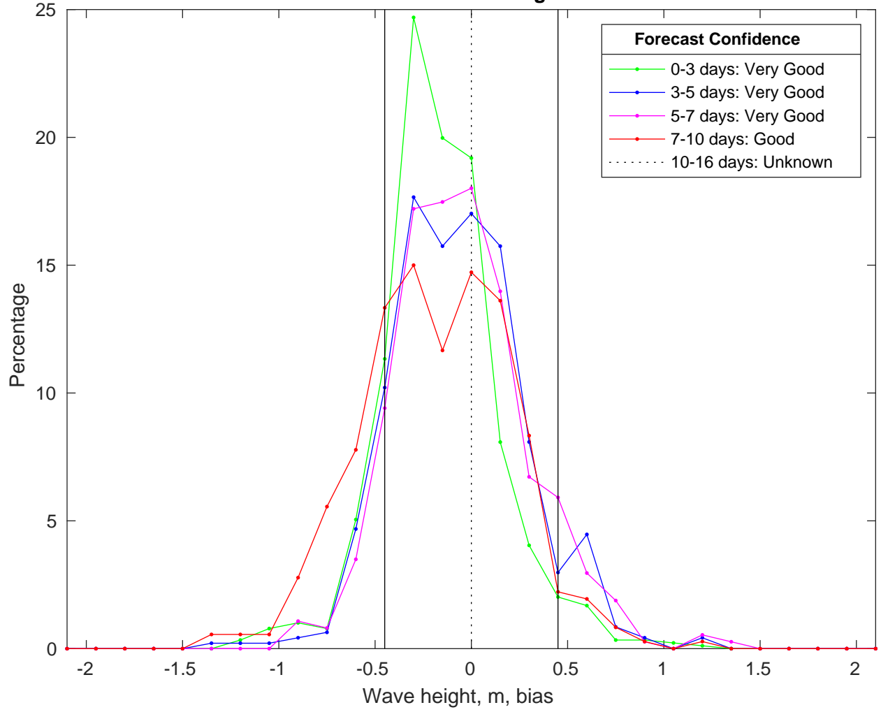
NDBC 46028 vs CMEMSWaves Bias Histogram: 11-Jan-2025
