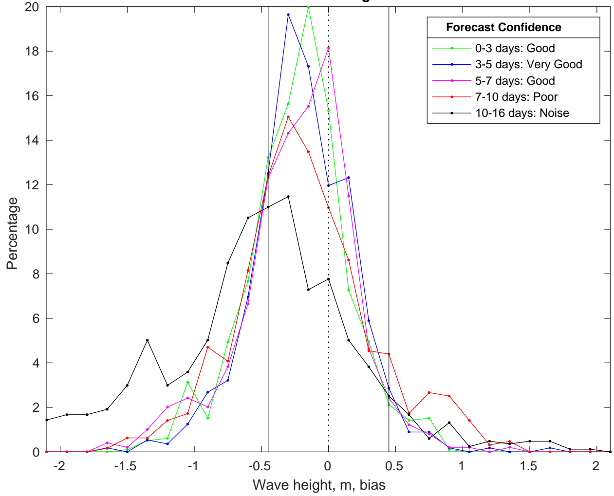
NDBC 46028 vs GFSWaves Bias Histogram: 11-Jan-2025
