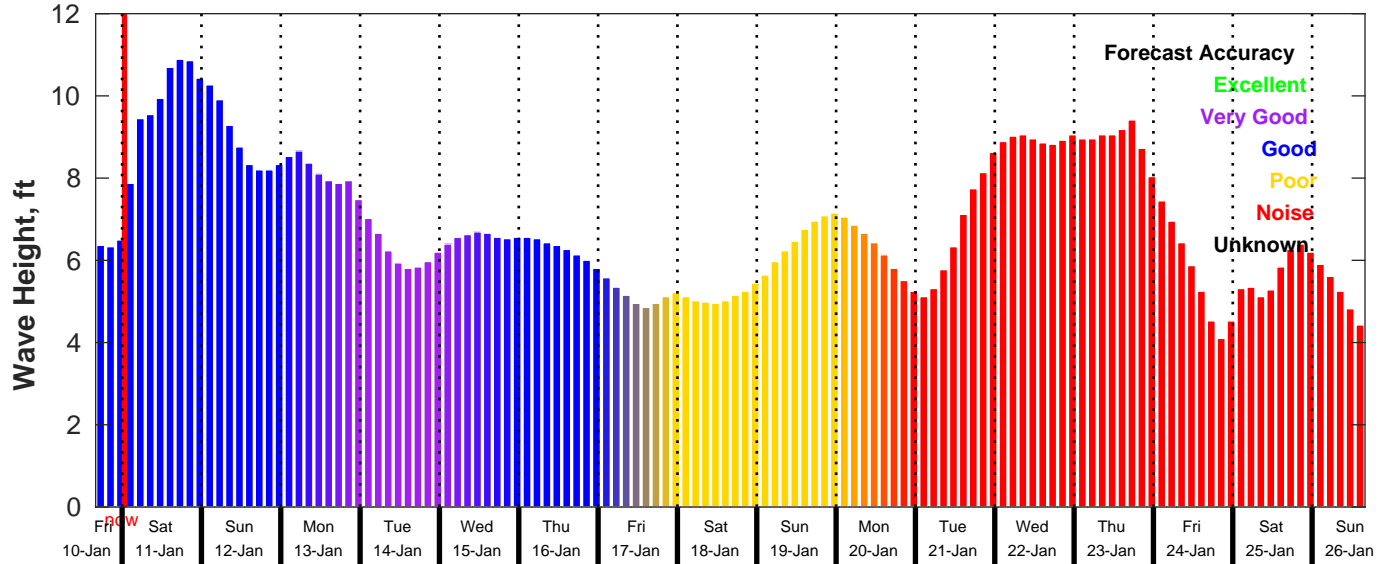
GFS Wave Forecast for NDBC 46028 from 10-Jan-2025 16:00:00 to 26-Jan-2025 16:00:00
