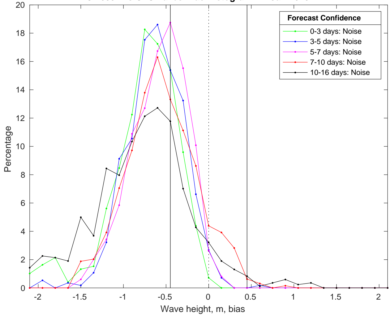
NDBC 46054 vs GFSWaves Bias Histogram: 11-Jan-2025
