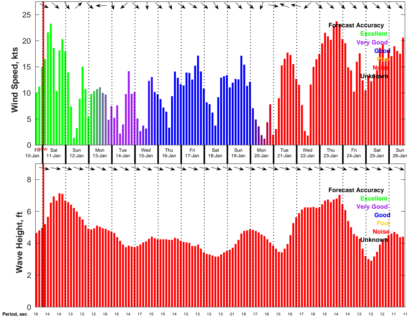
Wind & Wave Forecast for NDBC 46054 from 10-Jan-2025 16:00:00 to 26-Jan-2025 16:00:00
