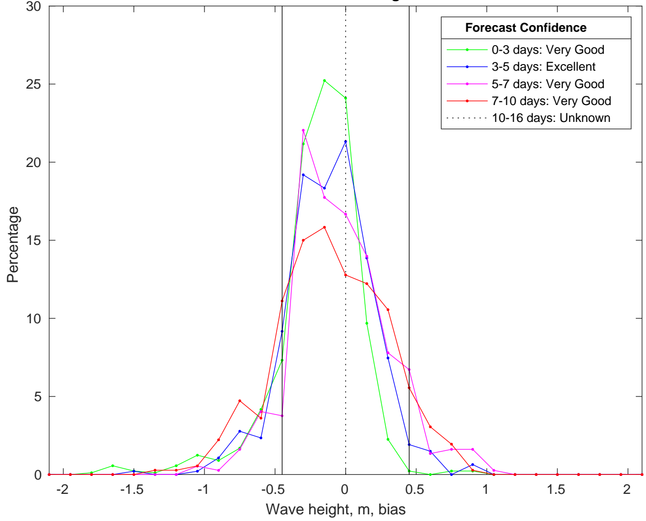
NDBC 46069 vs CMEMSWaves Bias Histogram: 11-Jan-2025
