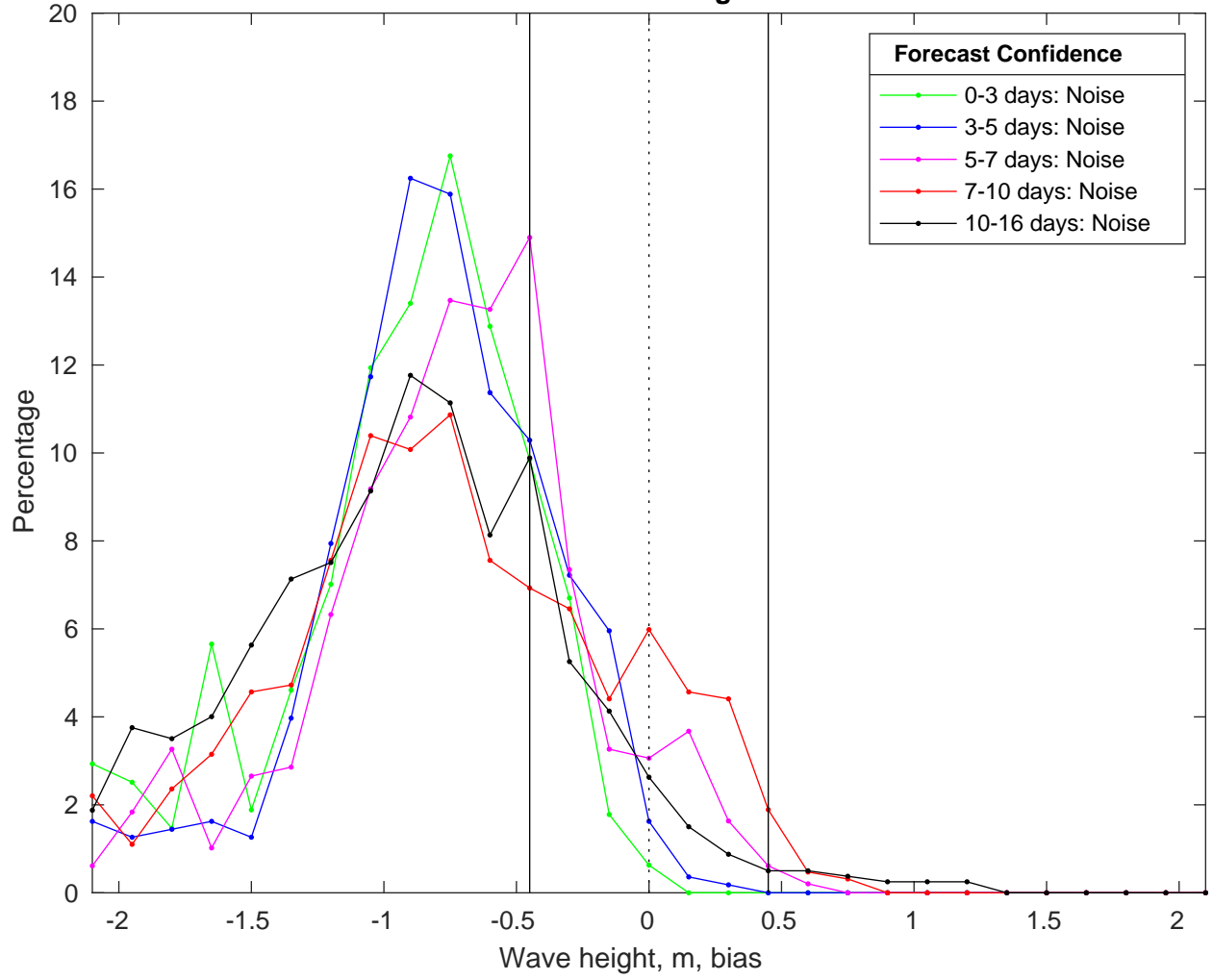
NDBC 46069 vs GFSWaves Bias Histogram: 11-Jan-2025
