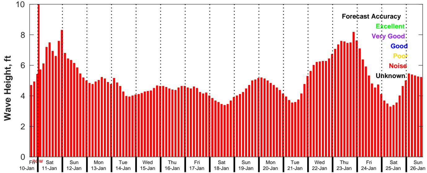
GFS Wave Forecast for NDBC 46069 from 10-Jan-2025 16:00:00 to 26-Jan-2025 16:00:00
