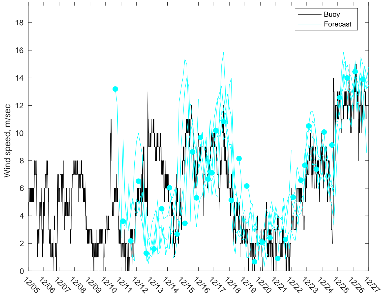
NDBC 46069 vs GFSWinds: 5 to 7 day forecast
