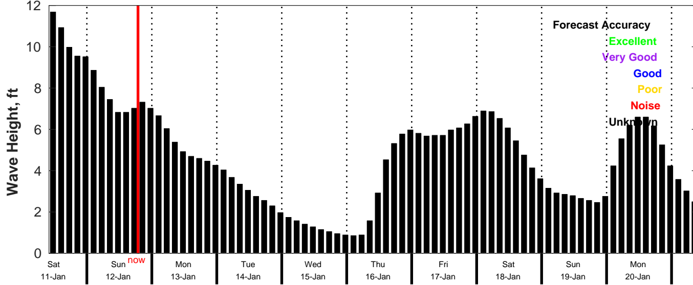
CMEMS Wave Forecast for NDBC 46246 from 10-Jan-2025 10:00:00 to 20-Jan-2025 10:00:00
