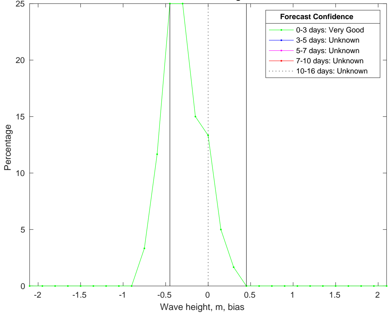
NDBC 51209 vs CMEMSWaves Bias Histogram: 11-Jan-2025
