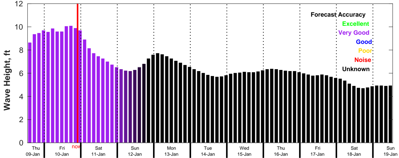
CMEMS Wave Forecast for NDBC 51209 from 09-Jan-2025 13:00:00 to 19-Jan-2025 13:00:00
