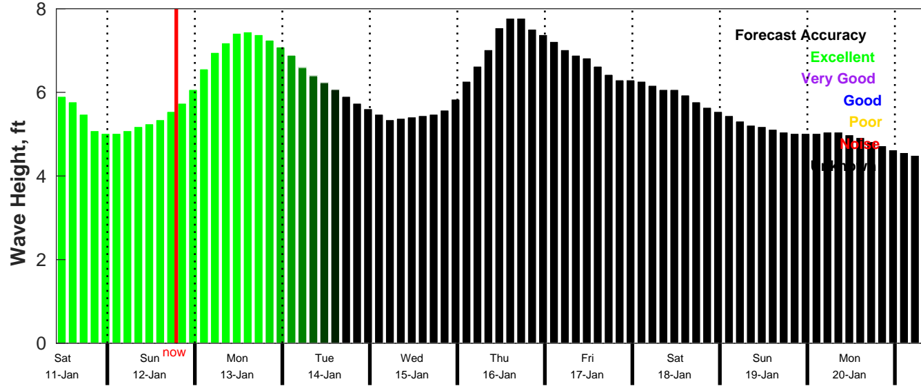
CMEMS Wave Forecast for NDBC 52211 from 10-Jan-2025 10:00:00 to 20-Jan-2025 10:00:00
