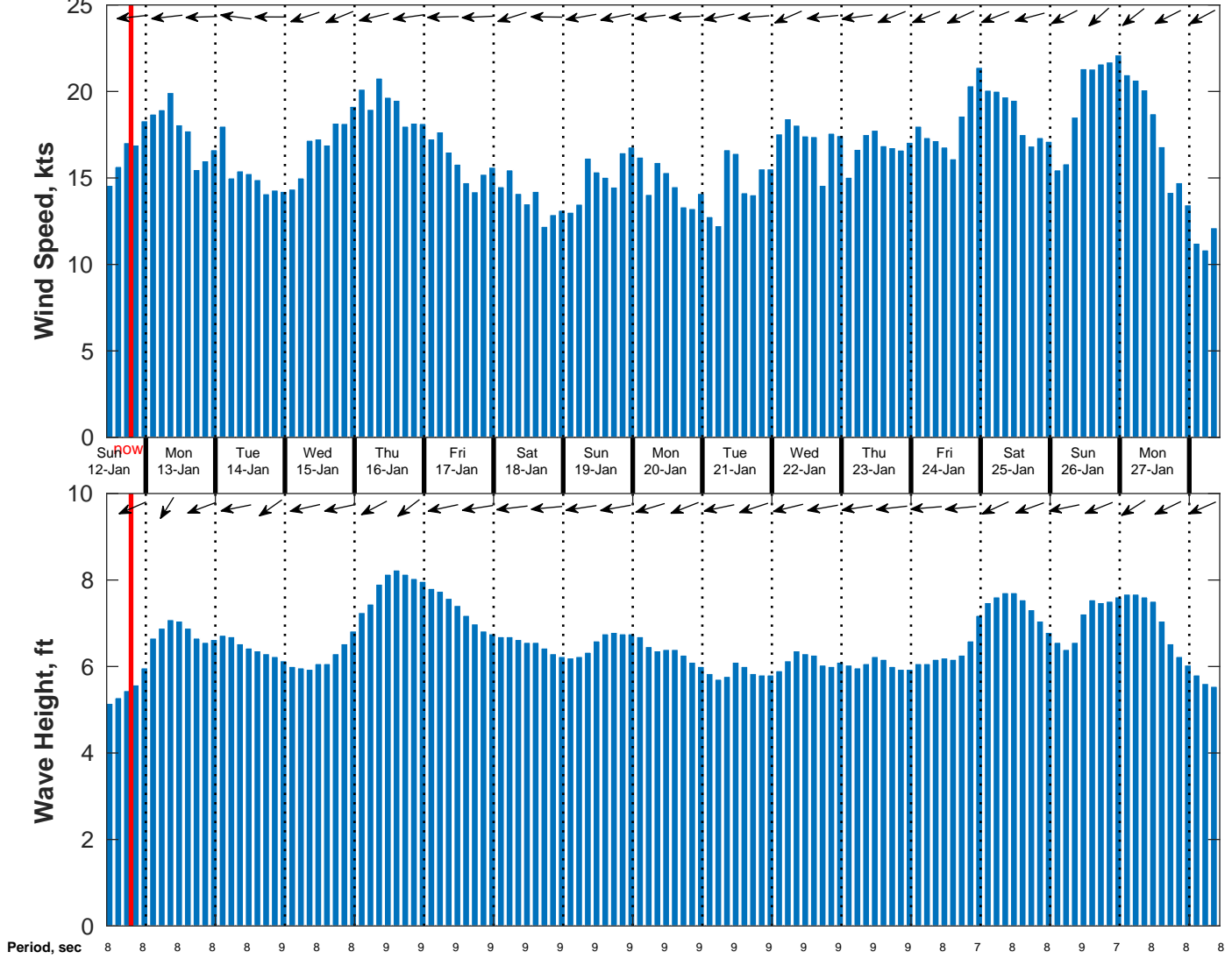
Wind & Wave Forecast for NDBC 52211 from 11-Jan-2025 10:00:00 to 27-Jan-2025 10:00:00
