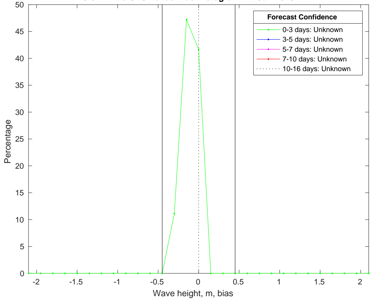
NDBC 52212 vs GFSWaves Bias Histogram: 11-Jan-2025
