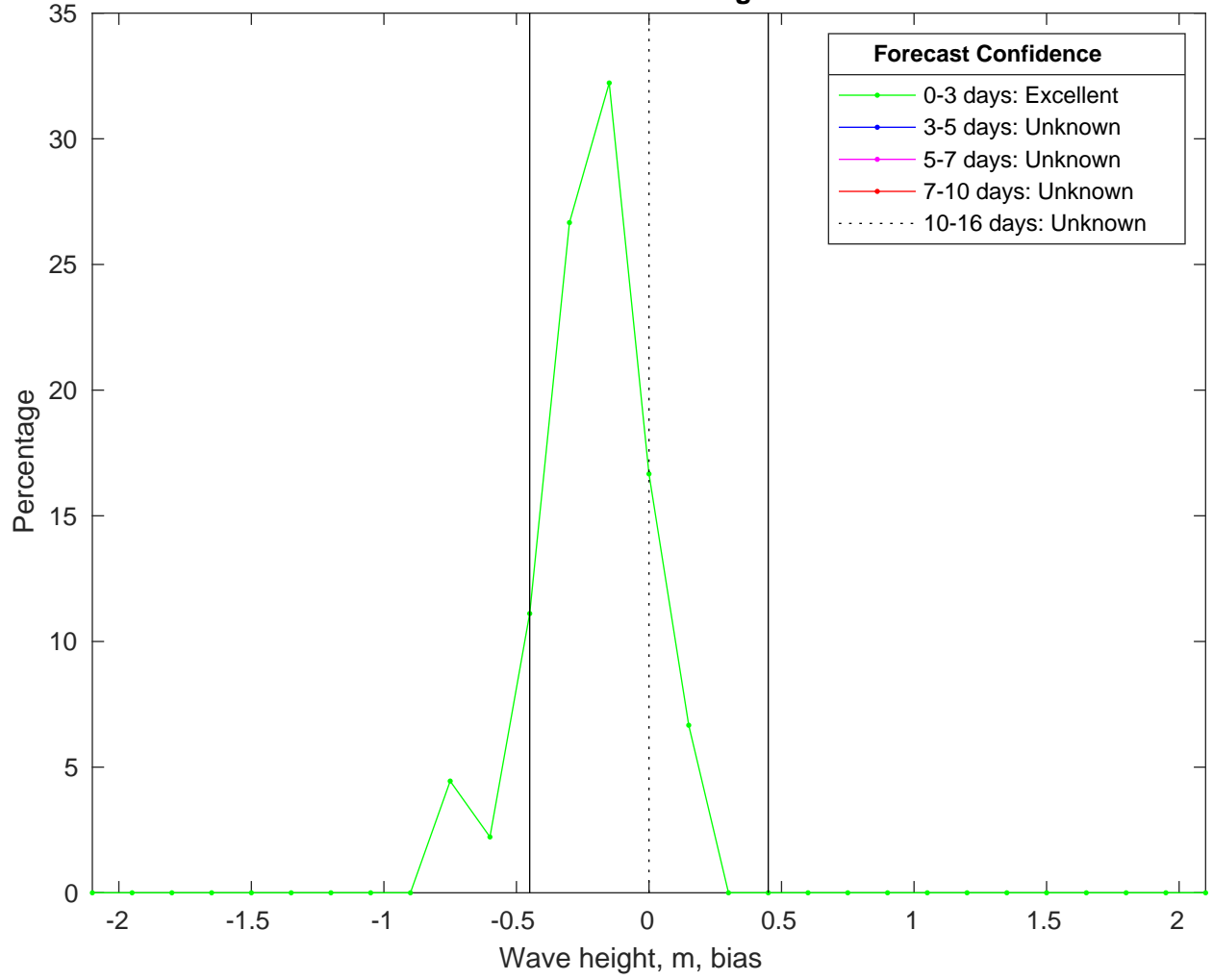
NDBC 52213 vs CMEMSWaves Bias Histogram: 11-Jan-2025
