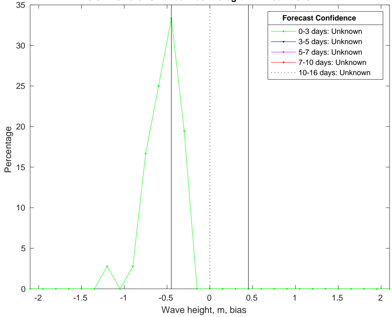
NDBC 52213 vs GFSWaves Bias Histogram: 11-Jan-2025
