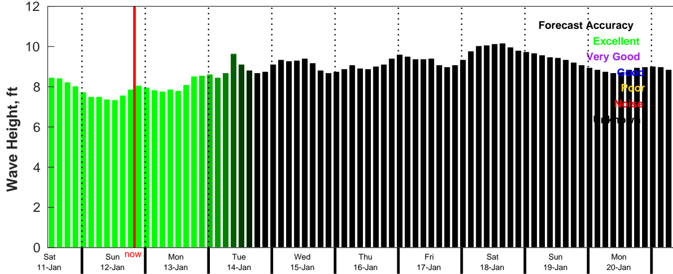
CMEMS Wave Forecast for NDBC 52213 from 10-Jan-2025 11:00:00 to 20-Jan-2025 11:00:00
