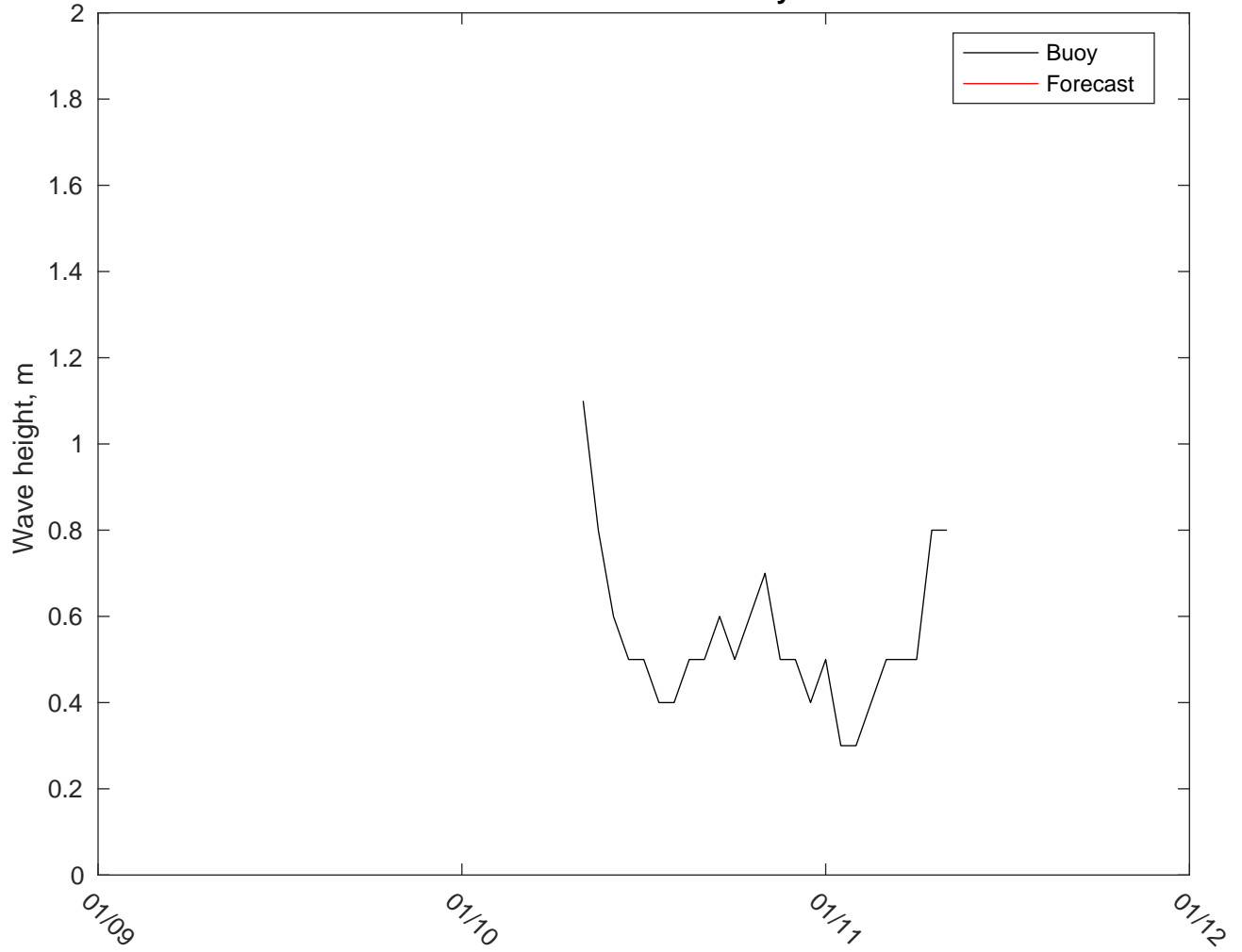
NDBC 62305 vs GFSWaves: 10 to 16 day forecast
