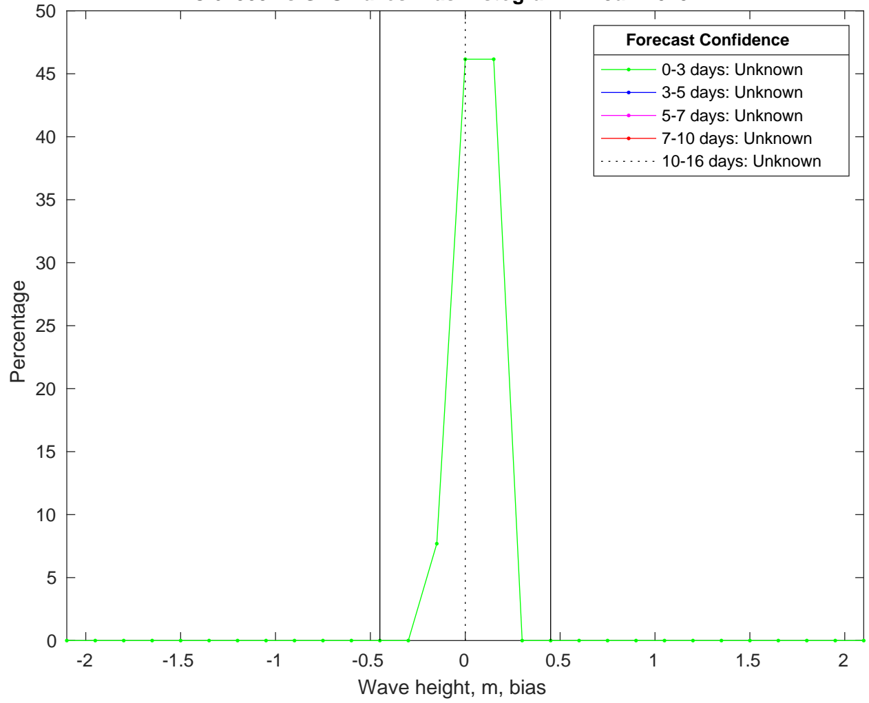
NDBC 62305 vs GFSWaves Bias Histogram: 11-Jan-2025
