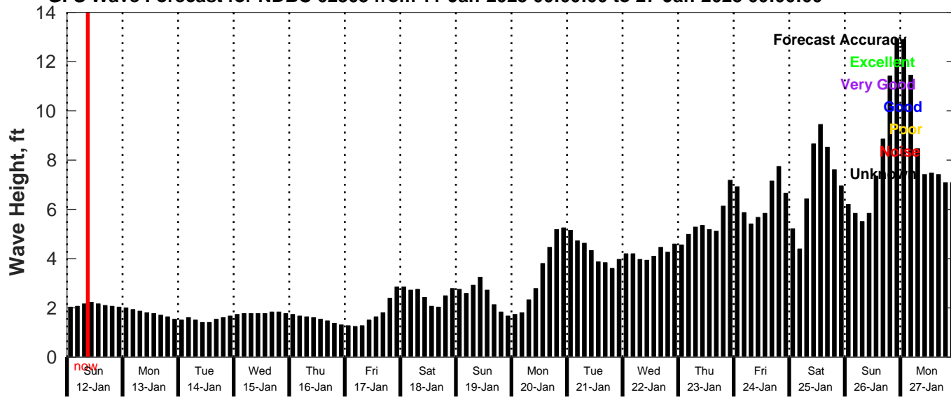
GFS Wave Forecast for NDBC 62305 from 11-Jan-2025 00:00:00 to 27-Jan-2025 00:00:00
