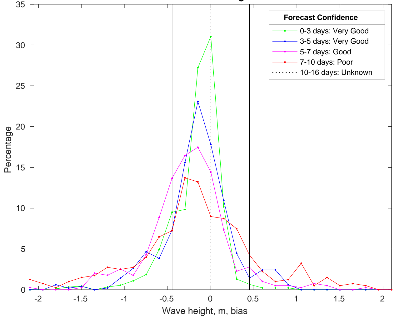
NDBC 41004 vs CMEMSWaves Bias Histogram: 12-Jan-2025
