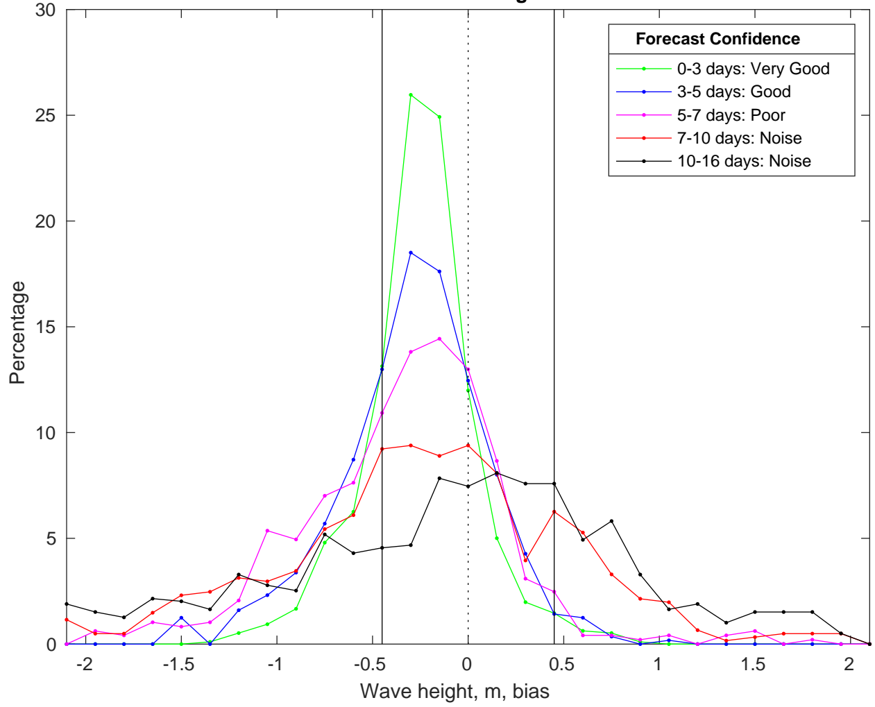
NDBC 41004 vs GFSWaves Bias Histogram: 12-Jan-2025
