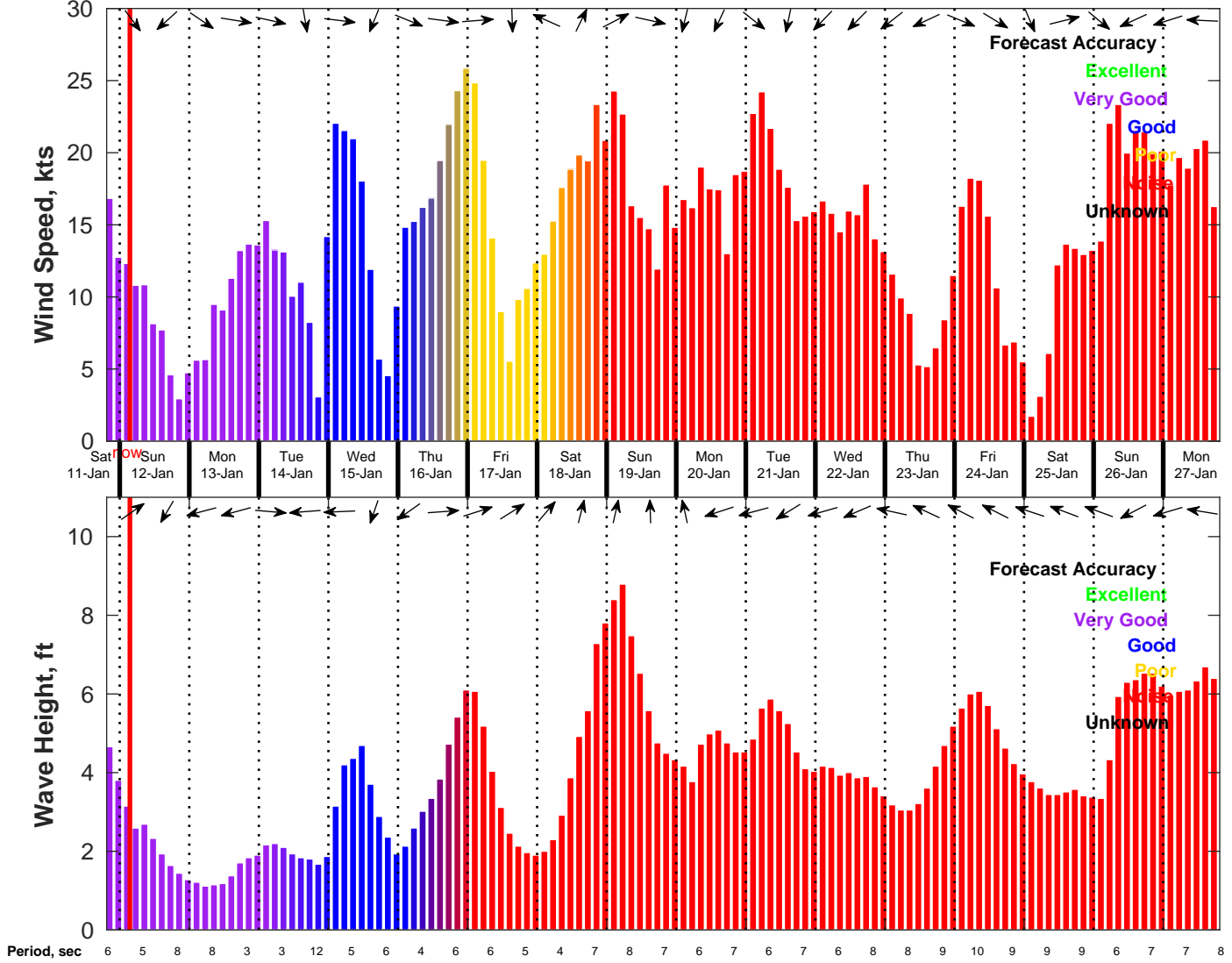
Wind & Wave Forecast for NDBC 41004 from 11-Jan-2025 19:00:00 to 27-Jan-2025 19:00:00
