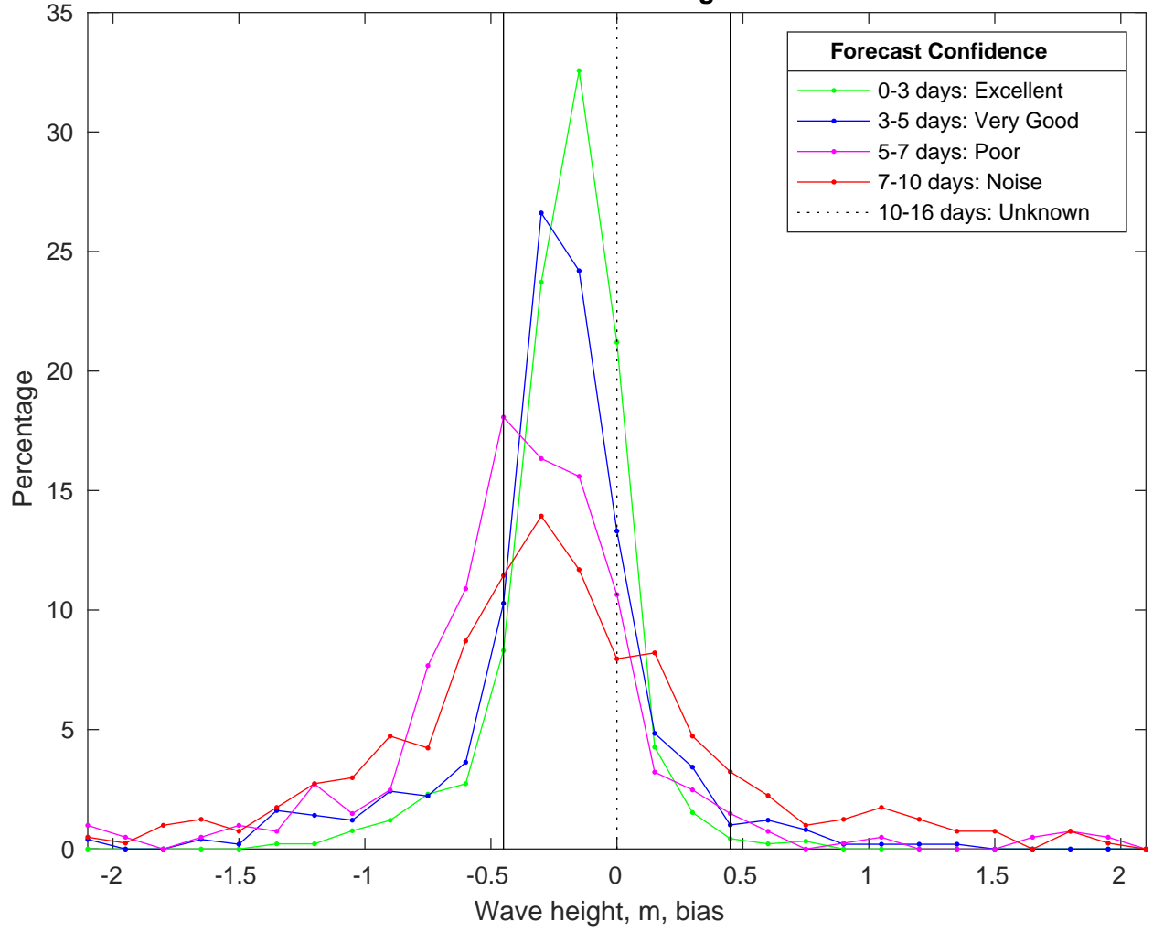
NDBC 41013 vs CMEMSWaves Bias Histogram: 12-Jan-2025
