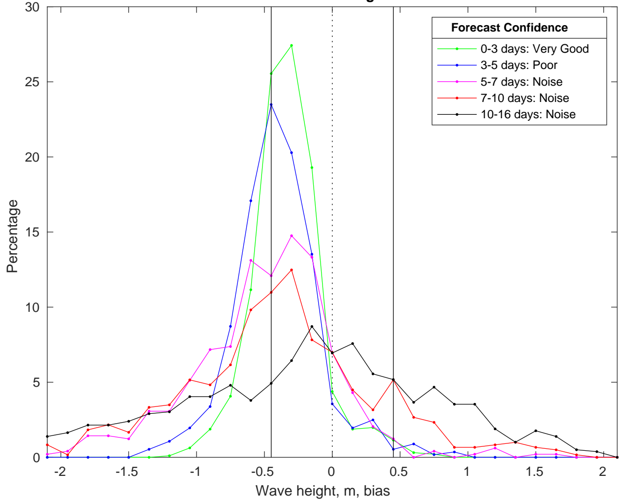
NDBC 41013 vs GFSWaves Bias Histogram: 12-Jan-2025
