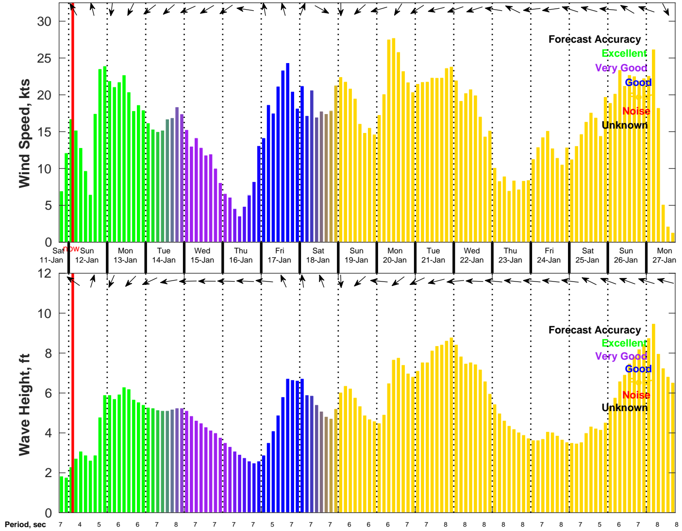
Wind & Wave Forecast for NDBC 42019 from 11-Jan-2025 18:00:00 to 27-Jan-2025 18:00:00
