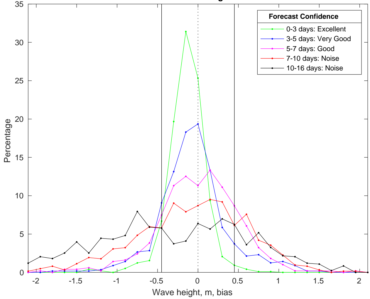
NDBC 42020 vs GFSWaves Bias Histogram: 12-Jan-2025
