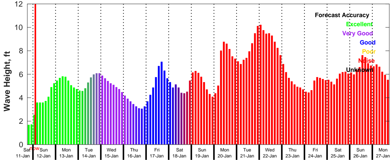
GFS Wave Forecast for NDBC 42020 from 11-Jan-2025 18:00:00 to 27-Jan-2025 18:00:00
