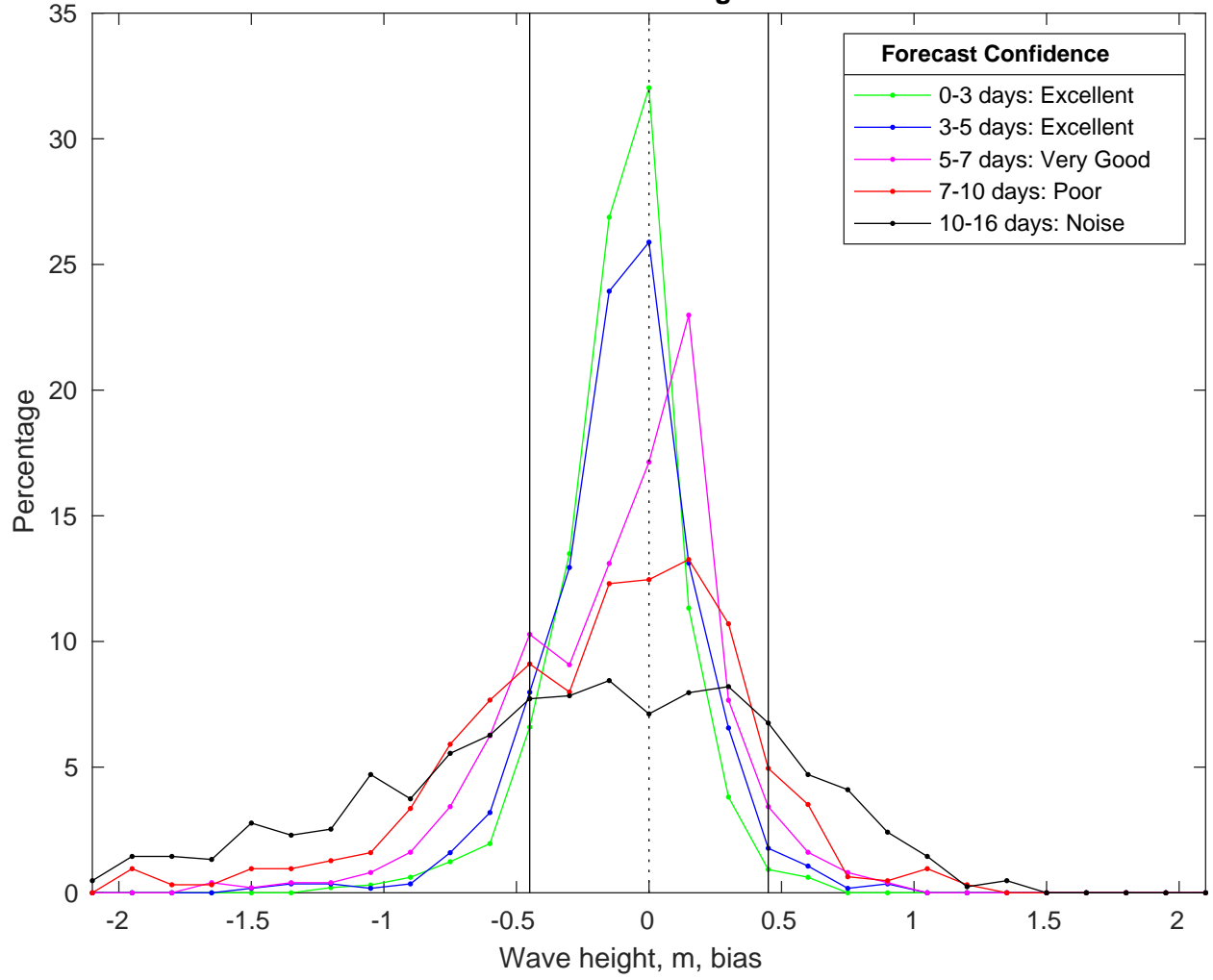
NDBC 42035 vs GFSWaves Bias Histogram: 12-Jan-2025
