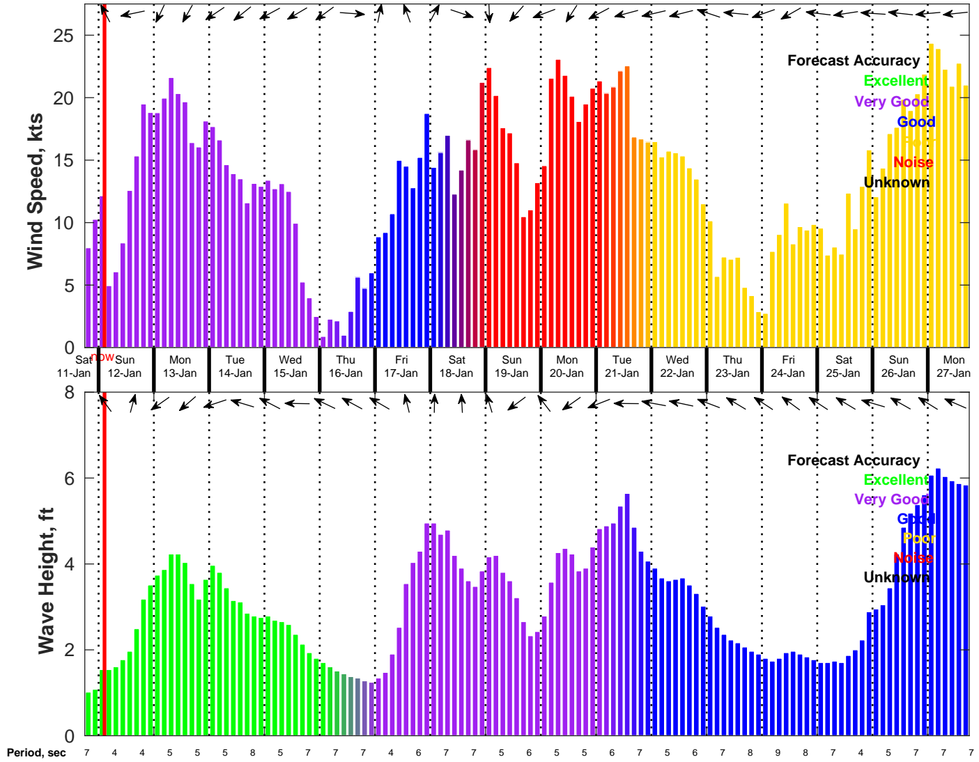
Wind & Wave Forecast for NDBC 42035 from 11-Jan-2025 18:00:00 to 27-Jan-2025 18:00:00
