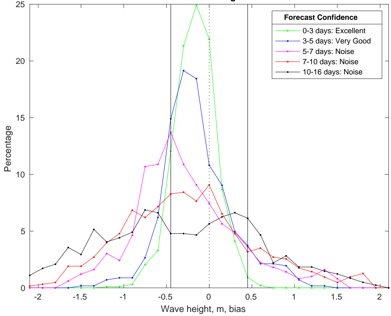
NDBC 42036 vs GFSWaves Bias Histogram: 12-Jan-2025
